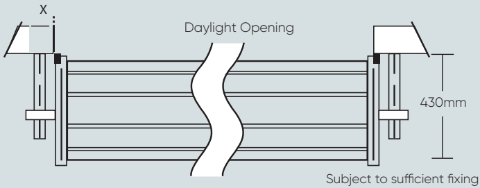
PLAN VIEW
